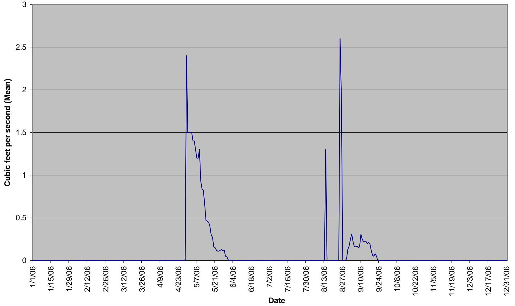
USGS Kings Creek Discharge (2006)
