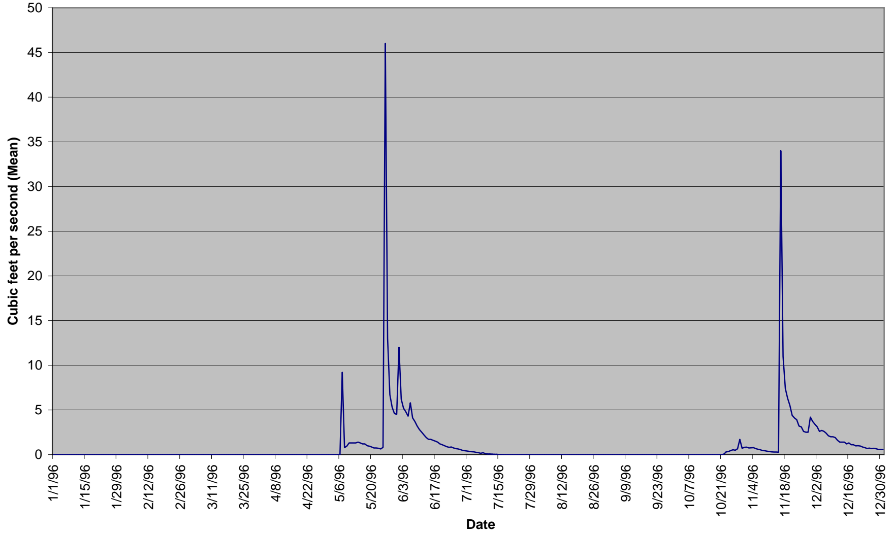
USGS Kings Creek Discharge (1996)
