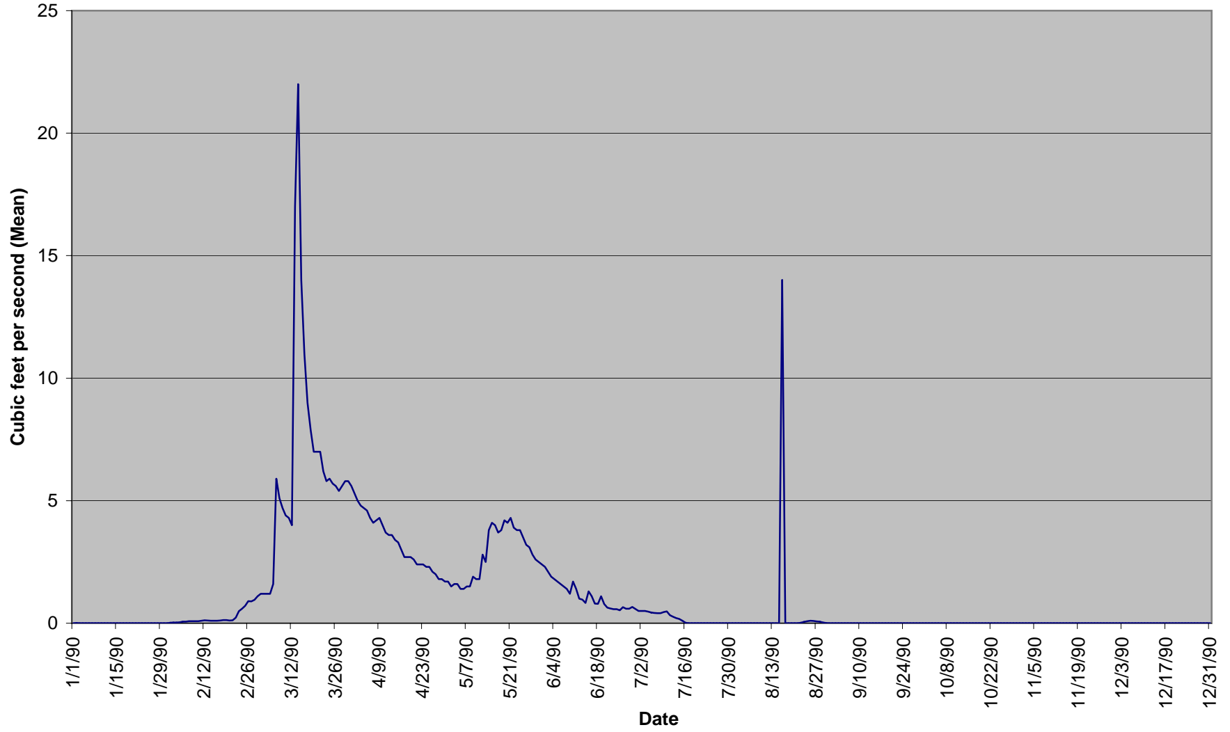
USGS Kings Creek Discharge (1990)
